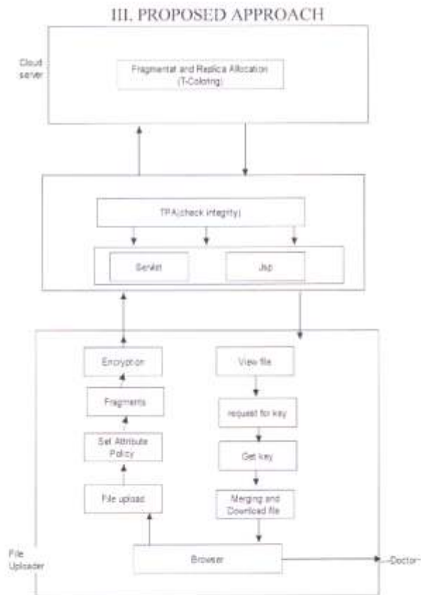
Fig 01: System Architecture
